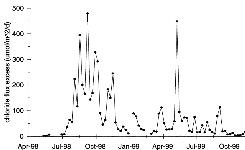
Figure 4. Post-cut difference in chloride flux between pine and bare sandboxes.
