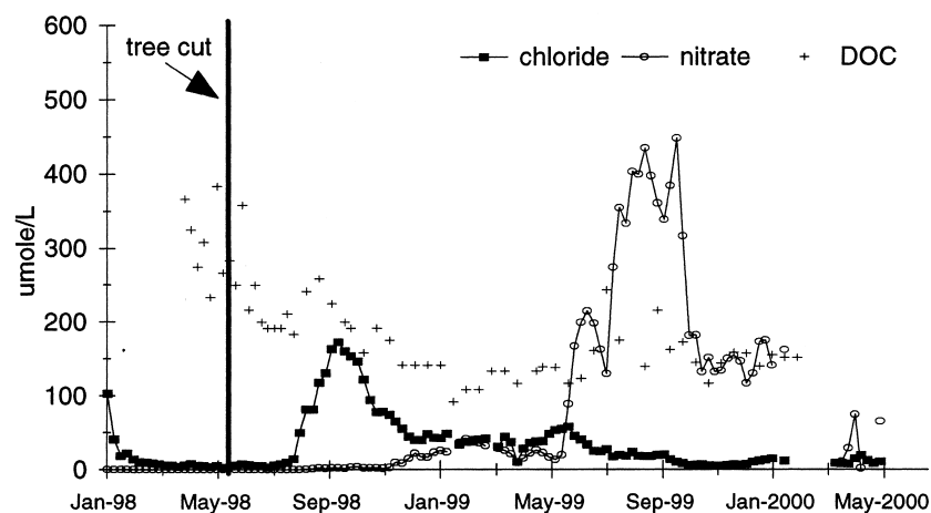
Figure 3. Chloride, nitrate and DOC concentrations in pine sandbox effluent.
