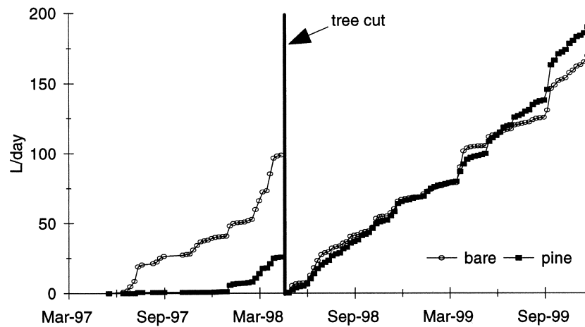
Figure 1. Cumulative discharge in pine sandbox before and after tree cut.
